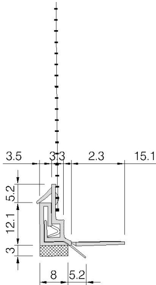
Alsipro SLIM - Dimensions in mm
