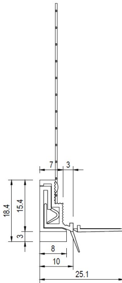
Alsipro SLIM - Maße in mm
